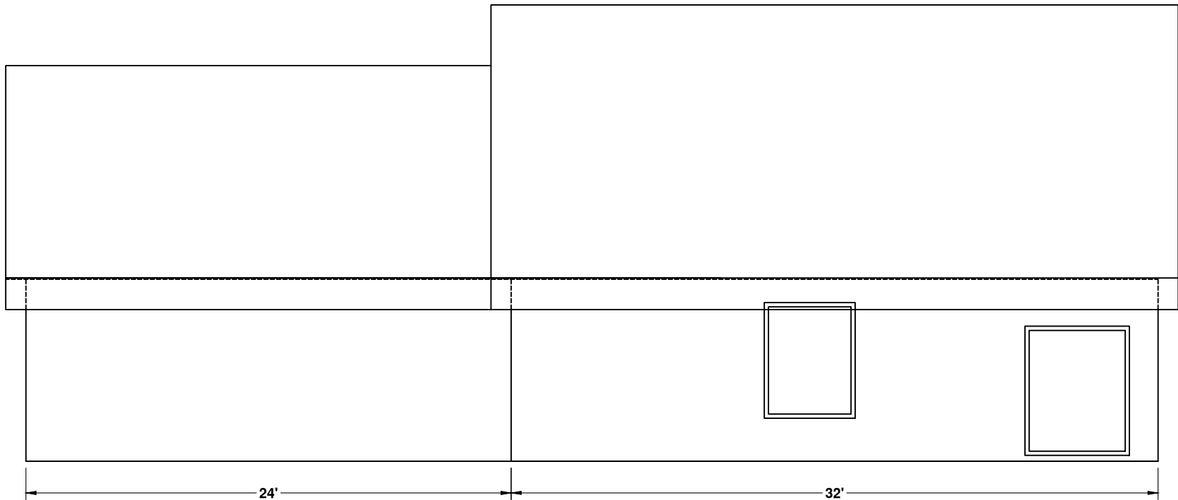
LEFT ELEVATION
