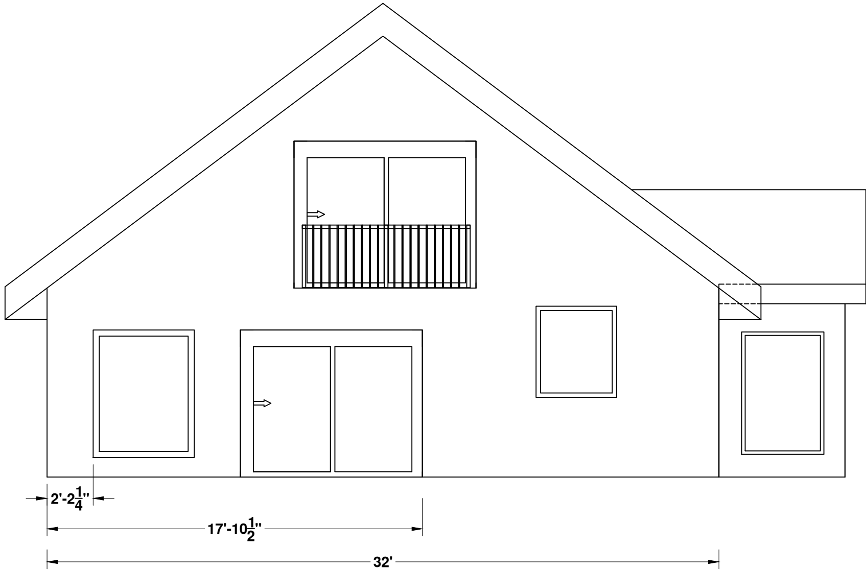
Front elevation 4
